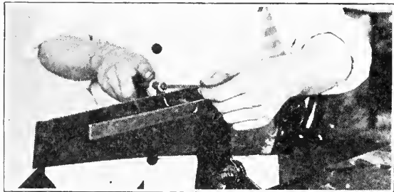
FIG. 113. FILING A CROSSCUT OR HANDSAW.
